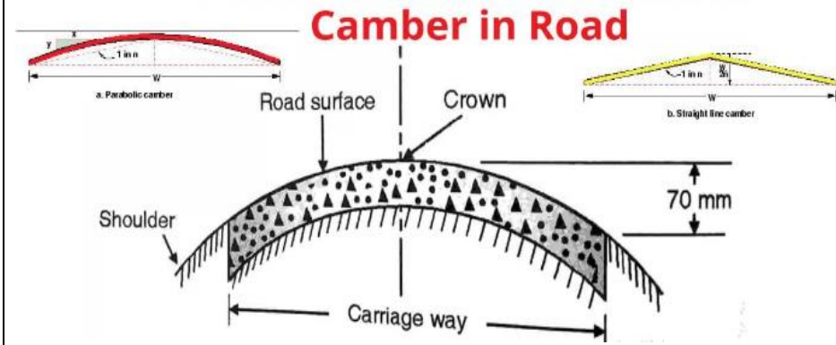
Fig. Camber in Road
